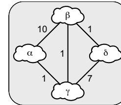
Received Path Vectors (1st exchange)
