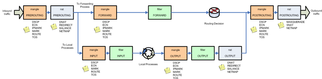
IPTables Chains Order Scheme
